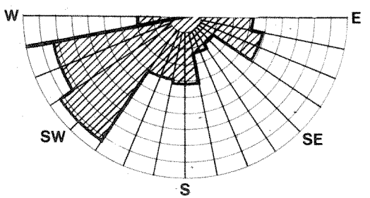
Offshore dominant fracture pattern
