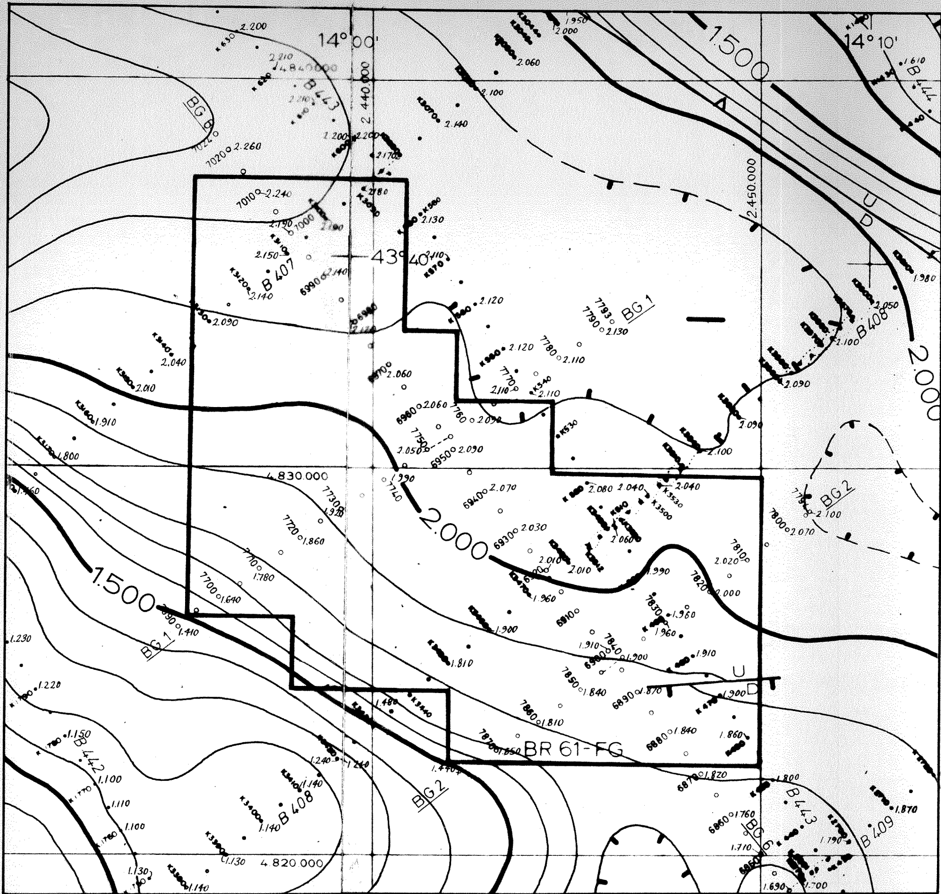
GULF ITALIA CO. ADRIATIC ZONE "B" - PERMIT "BR. 61-FG" SEISMIC CONTOURS ON TOP OF MAJOR MIOCENE UNCONFORMITY
