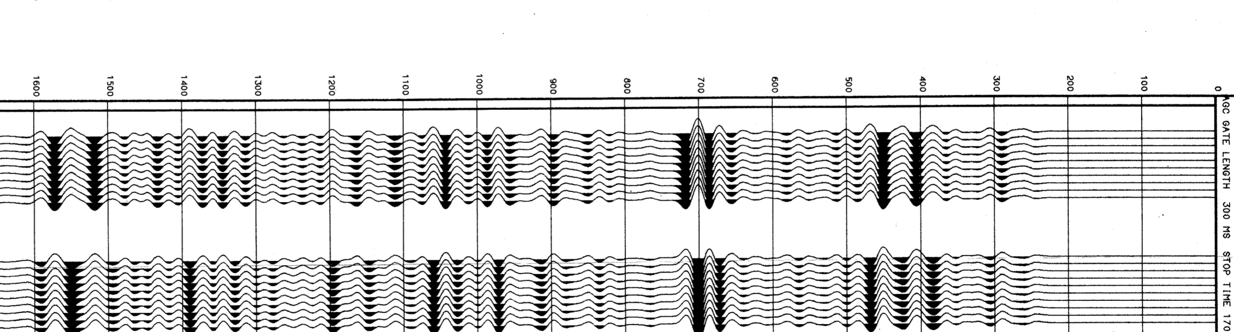
COZZO SCALIA 1 RICKER WAVELET 35 MS ZERO PHASE
