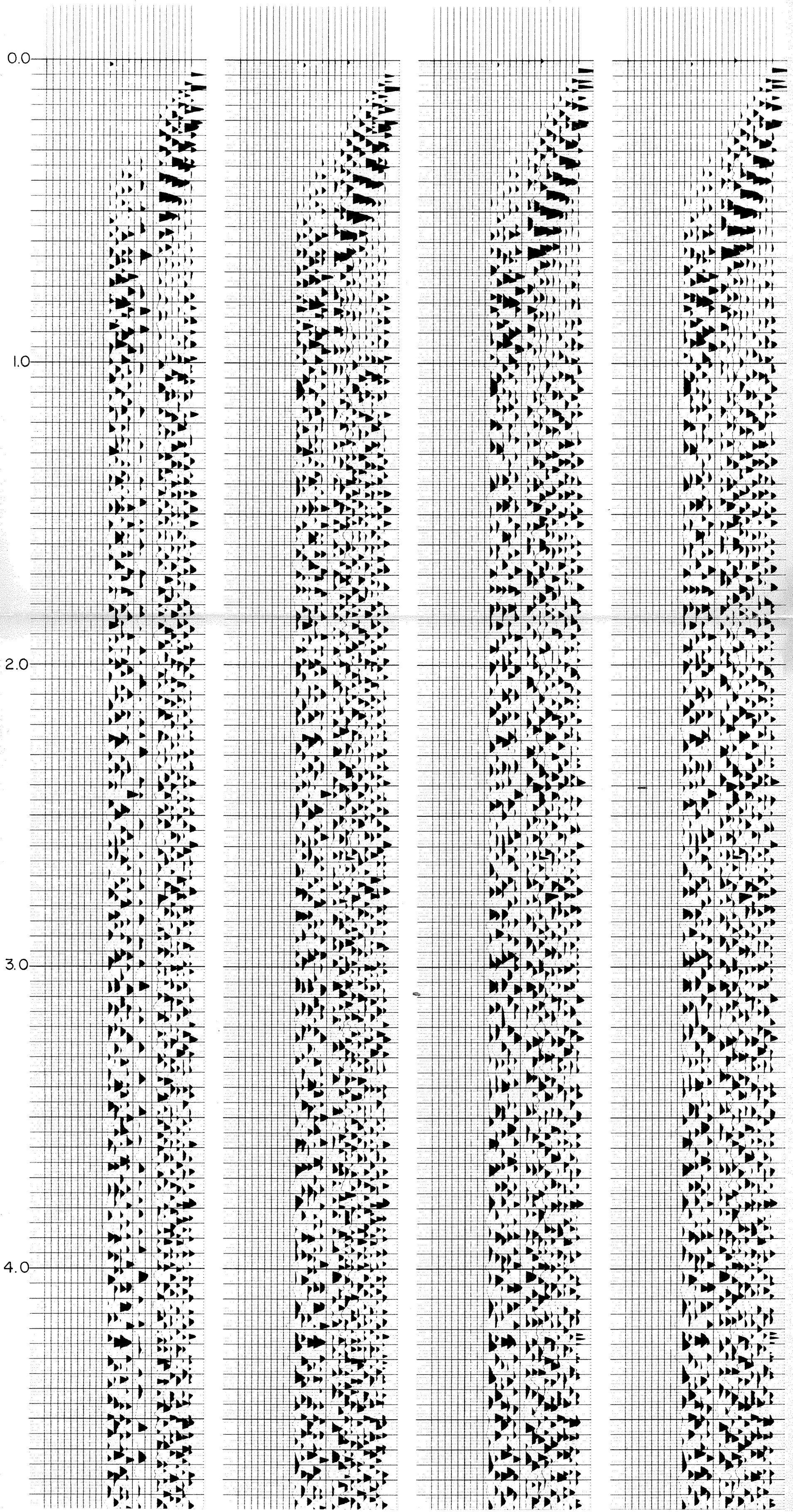
3 HOLE SHARGED pattern 15 GEOPHONES AT 120 m INTERVAL
