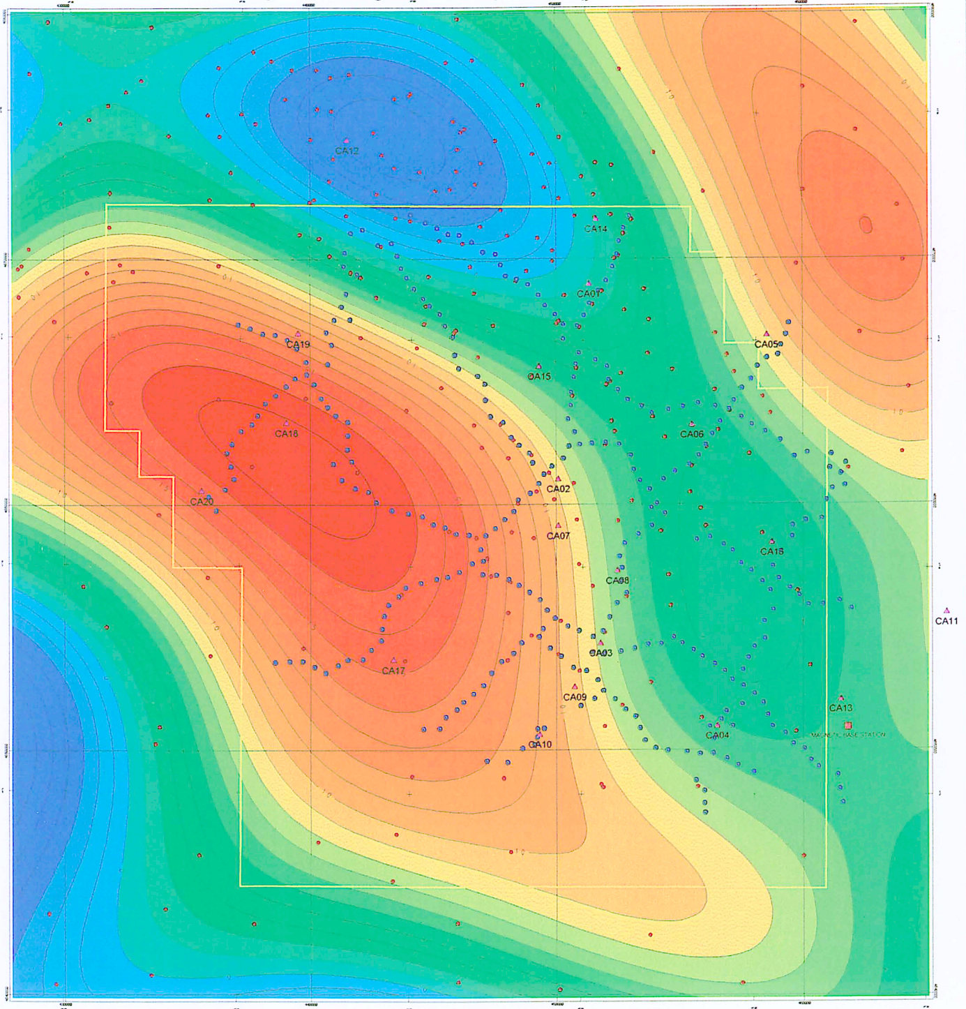
Figure 11) Regional Gravity Anomaly Map (mGal)
