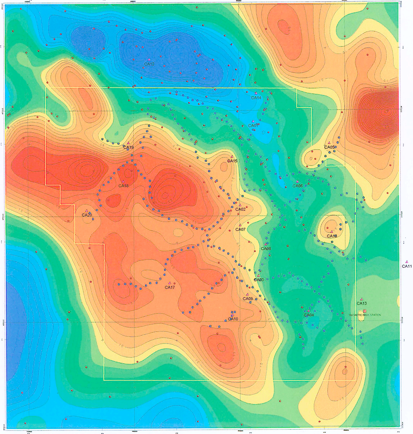
Figure 10) Isostatic Gravity Anomaly Map (mGal)
