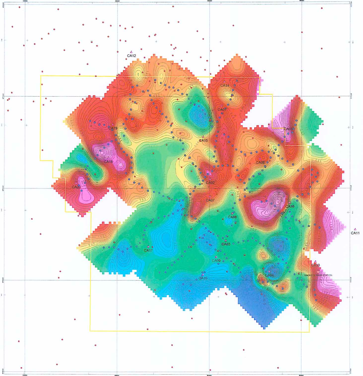
Figure 8) Reduced-to-Pole (RTP) Magnetic Anomaly Map (nT)
